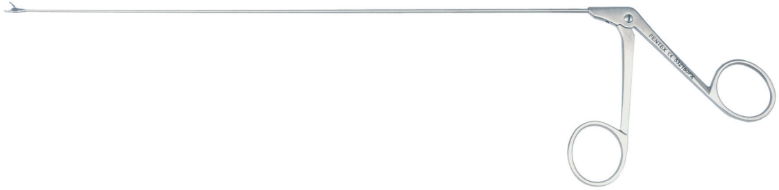
532160FX Laryngeal Biopsy Forceps , delicate, straight, round, WL 23 cm, Ø 1 mm Larynx Löffelzange , fein, gerade, rund, NL 23 cm, Ø 1 mm
